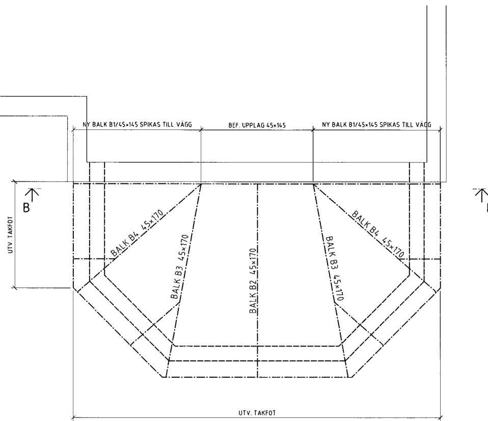
TAKPLAN -1:20-
